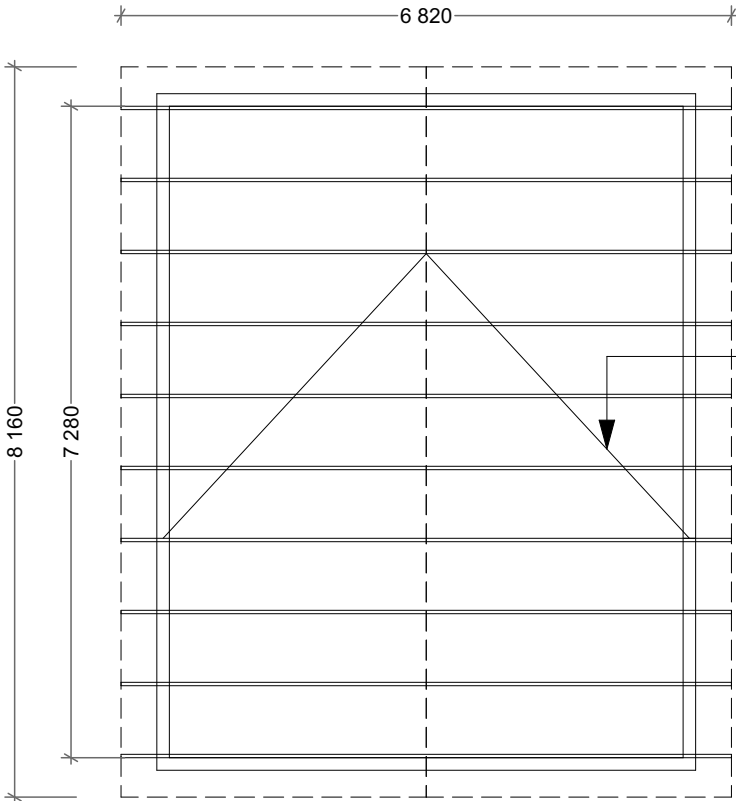
ROOF TRUSS PLAN SCALE 1: 100
