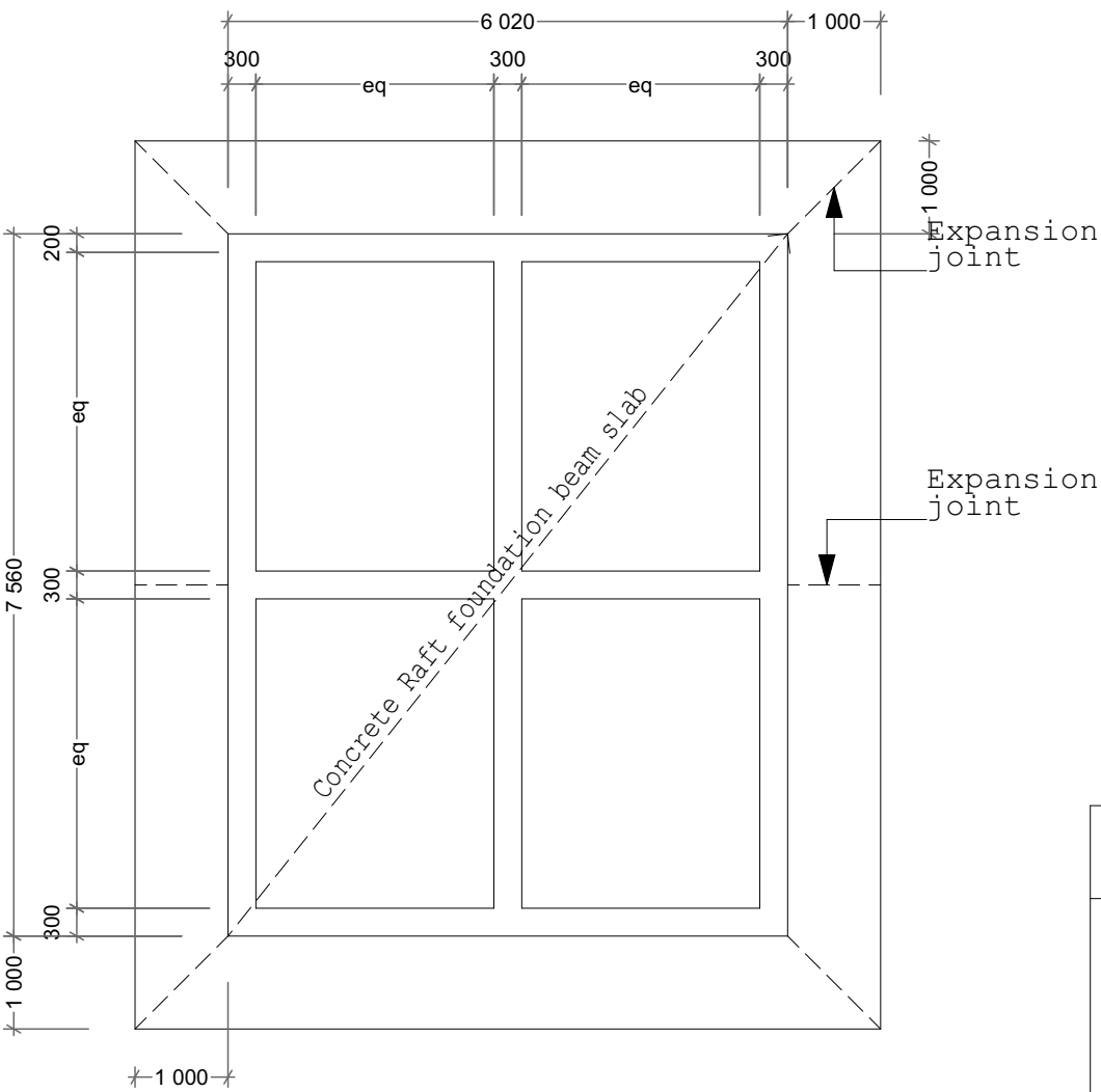
FOUNDATION PLAN SCALE 1: 100
