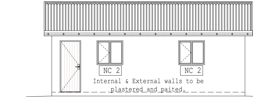
ELEVATION A SCALE 1: 100
